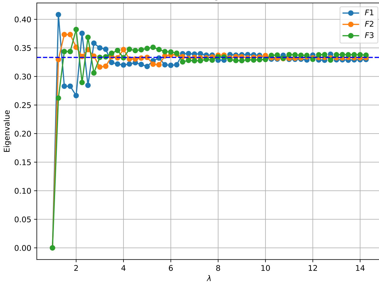
Measured eigenvalues
