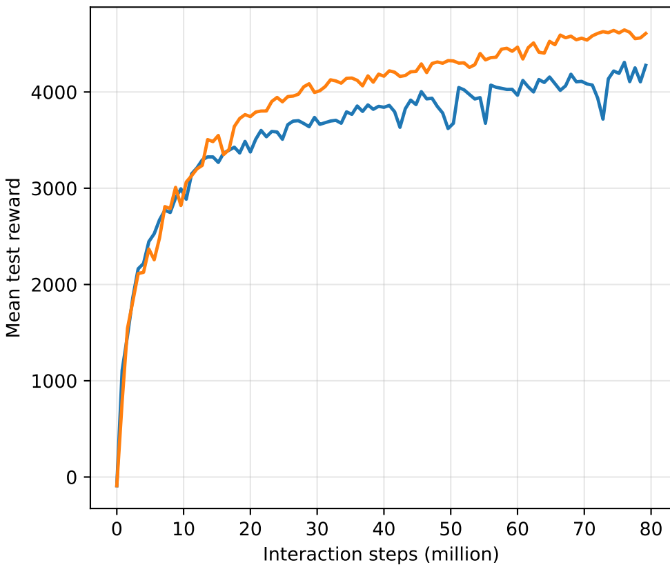
HalfCheetah-v5
