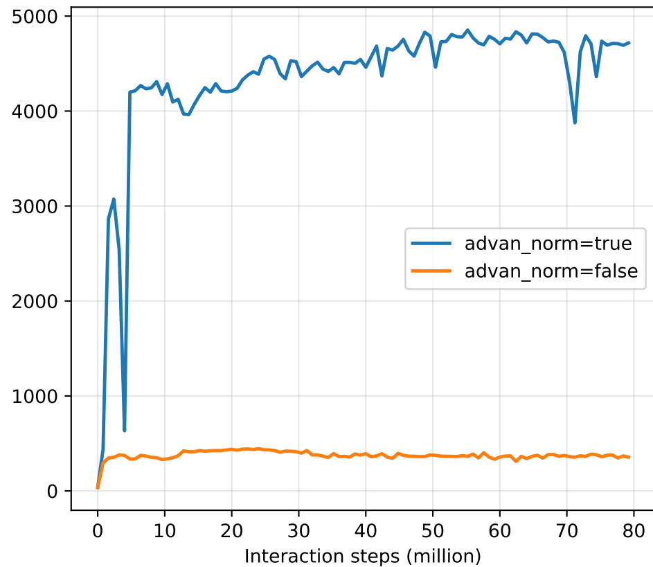
Walker2d-v5
