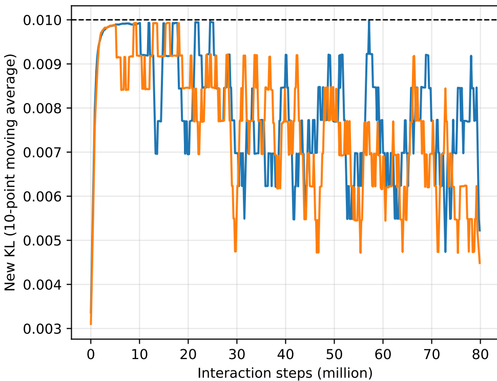
HalfCheetah-v5
