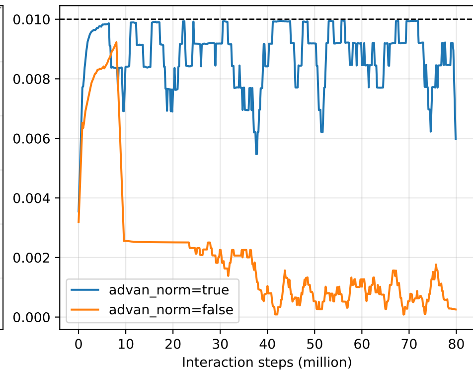
Walker2d-v5
