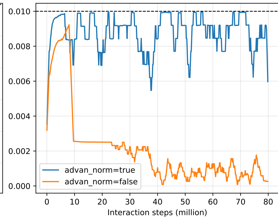
Walker2d-v5
