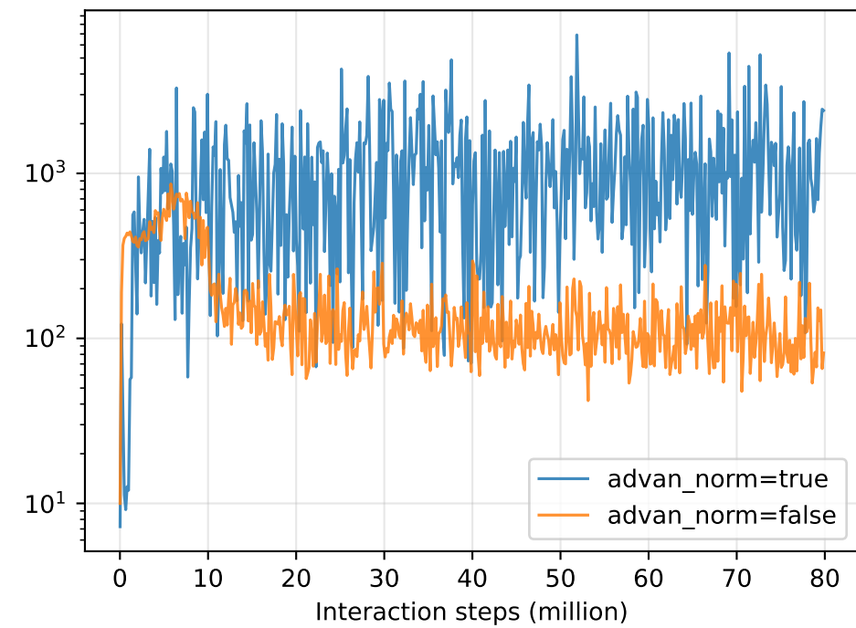
Walker2d-v5
