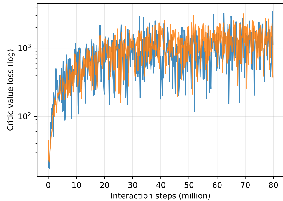
HalfCheetah-v5
