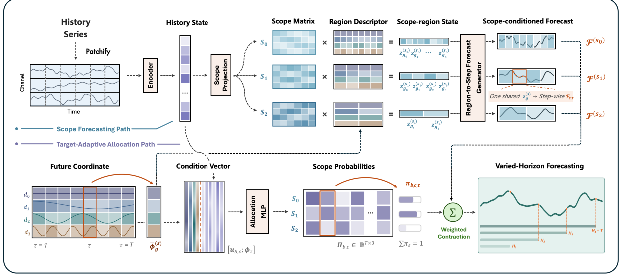
Figure 4: HoriScope for unified varied-horizon forecasting. The Scope Forecasting Path constructs region-wise forecasts under multiple scopes, and the Target-Adaptive Allocation Path combines them into one trajectory whose prefixes serve different horizon requests.
