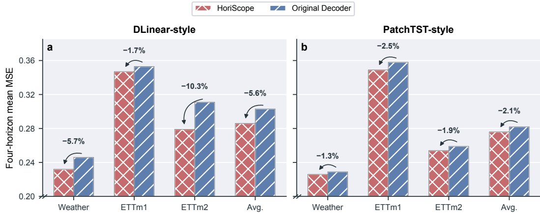
Figure 7: Generalization across two forecasting backbones. Four-horizon mean MSE is reported for a , DLinear and b , PatchTST with either the Original Decoder or HoriScope.
