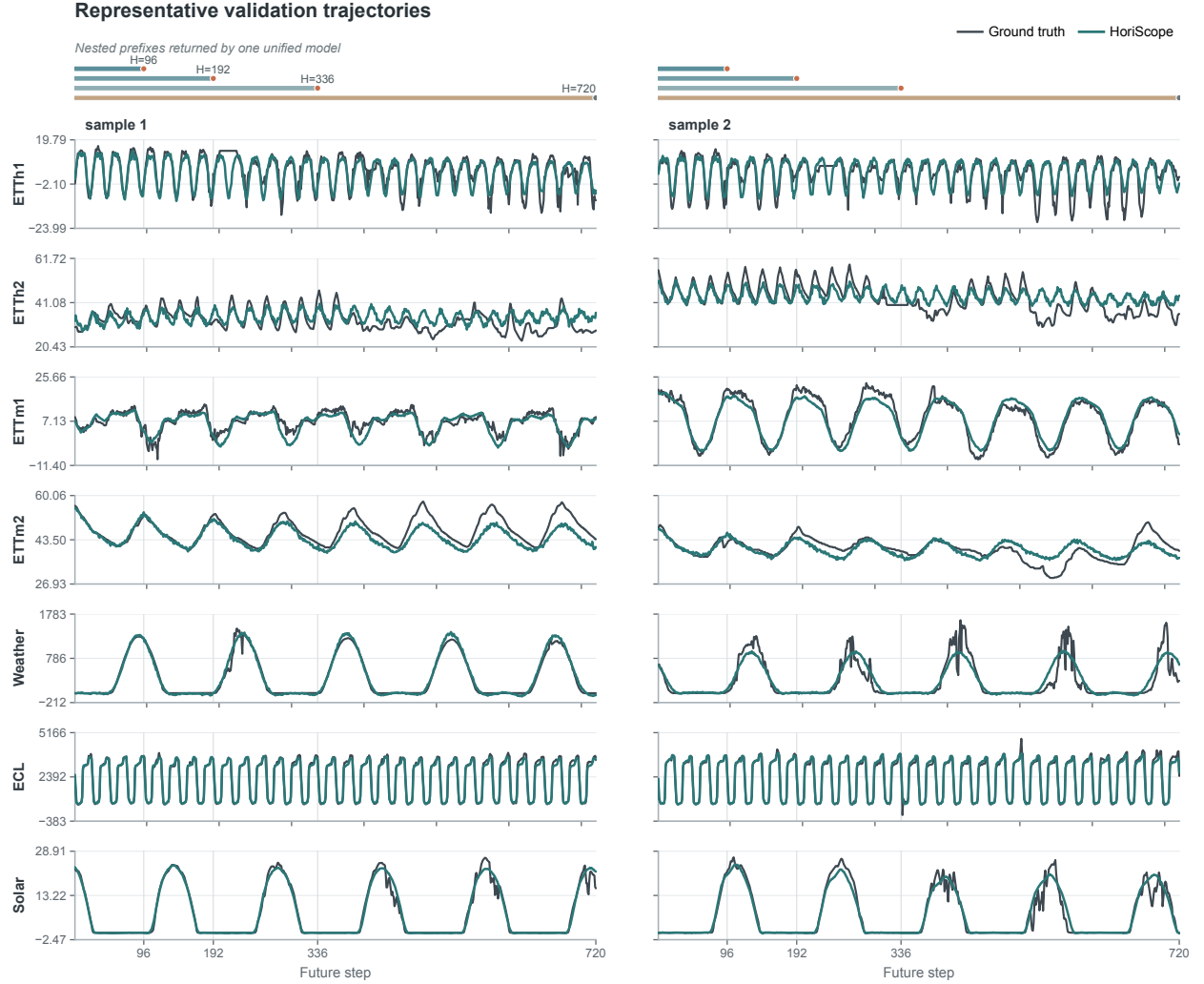
Figure C.1: Visualization of varied-horizon forecasts across seven datasets. The dark curve denotes the ground truth and the teal curve denotes the prediction from the frozen unified HoriScope model. Two validation examples are shown for each dataset. The paired rulers and vertical guides identify the four supported prediction lengths.
