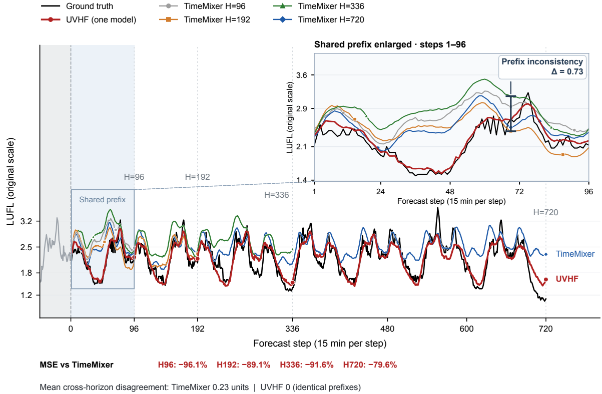
Figure 8: Forecasting performance and prefix consistency on a selected ETTm1 validation example. The black curve denotes the ground truth for LUFL, the red curve denotes UVHF, and the other curves denote independently trained TimeMixer models for H \in \{96, 192, 336, 720\} . The inset enlarges the shared first 96 steps. At step 69, \Delta is the range across the four TimeMixer predictions in the original data scale. MSE reductions compare UVHF with the corresponding TimeMixer model over each complete horizon. Mean cross-horizon disagreement averages the six pairwise mean absolute differences over their respective overlapping intervals for this variable. The example is selected for illustration, not to estimate average performance.
