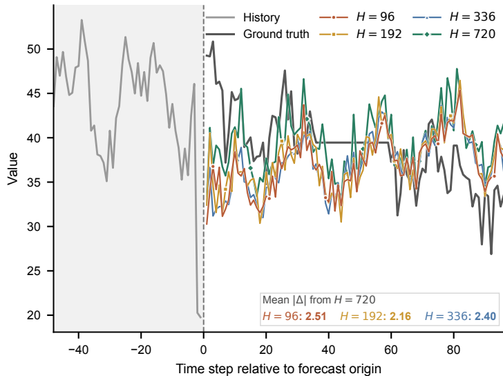
Same future steps, different horizon-specific forecasts
