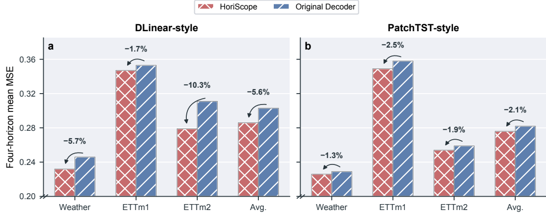
Figure 7: Generalization across two forecasting backbones. Four-horizon mean MSE is reported for a , DLinear and b , PatchTST with either the Original Decoder or HoriScope.
