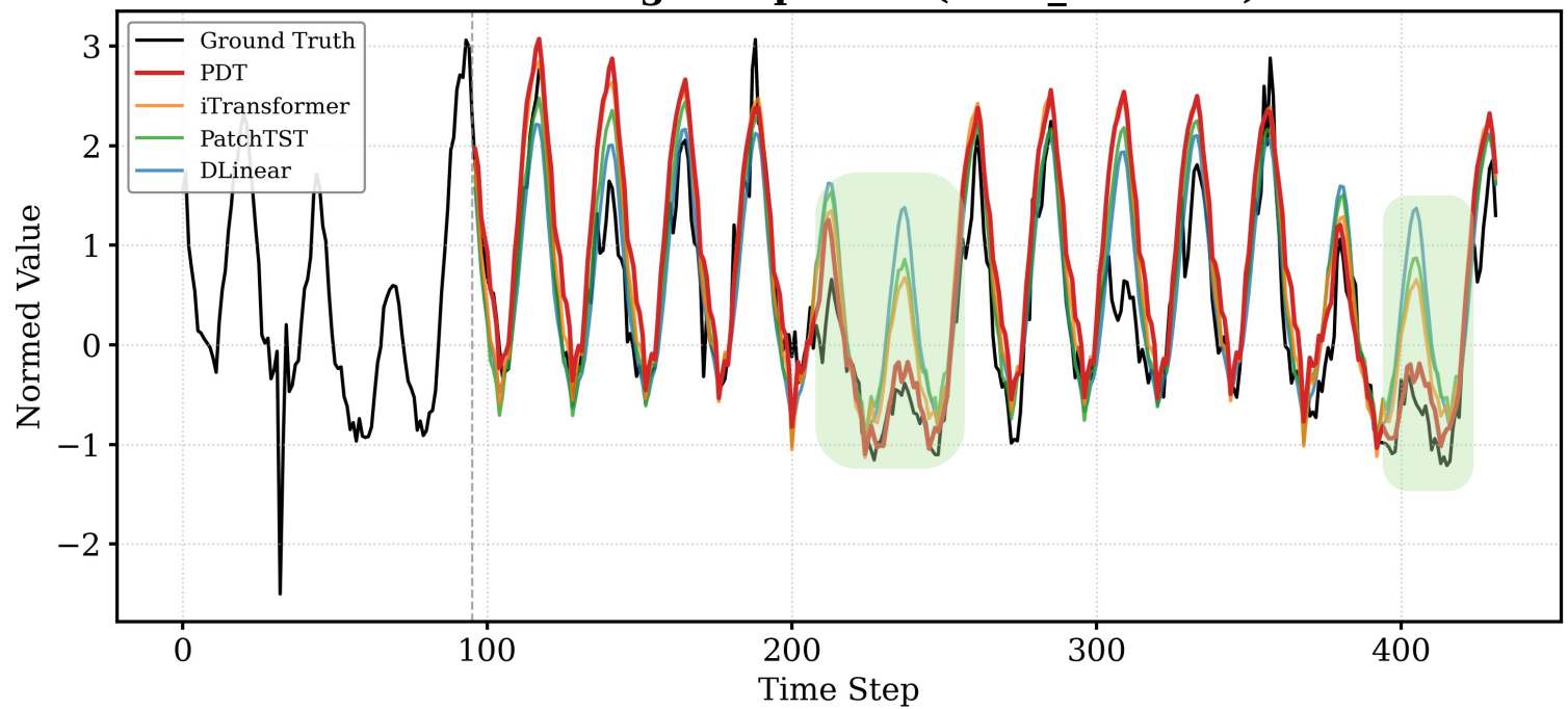
Forecasting Comparison(Pred_len=336)
