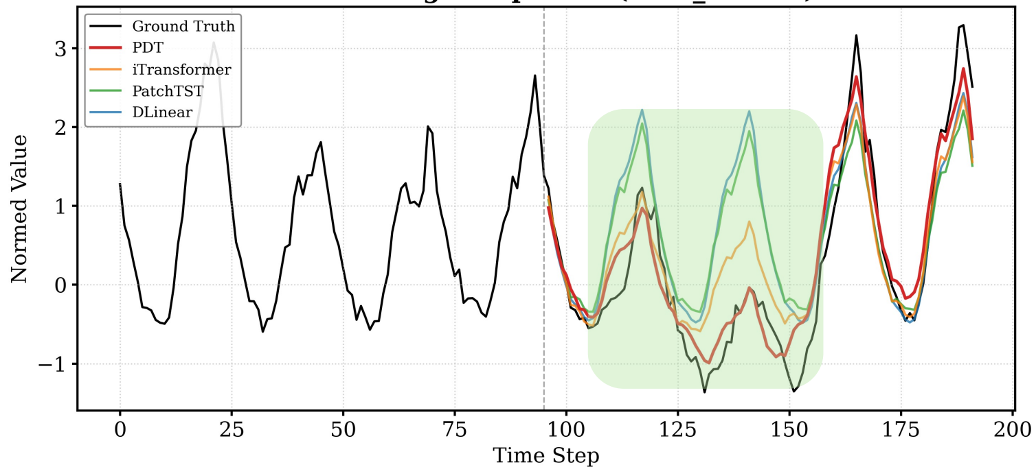
Forecasting Comparison(Pred_len=96)
