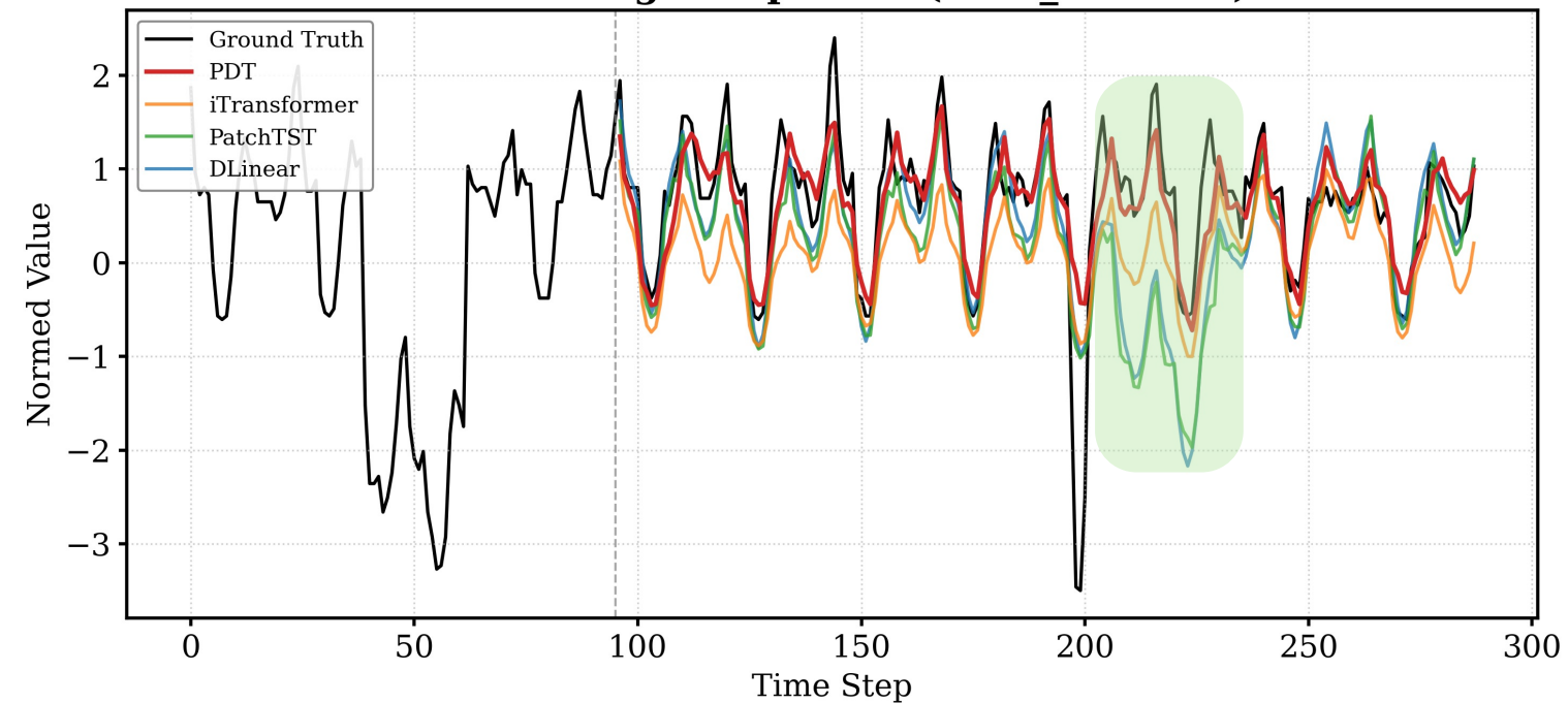
Forecasting Comparison(Pred_len=192)
