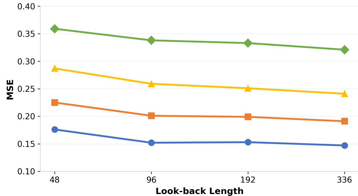
Weather
