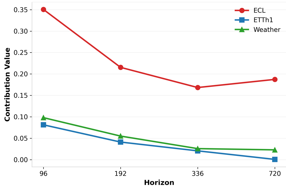
Encoder Contribution
