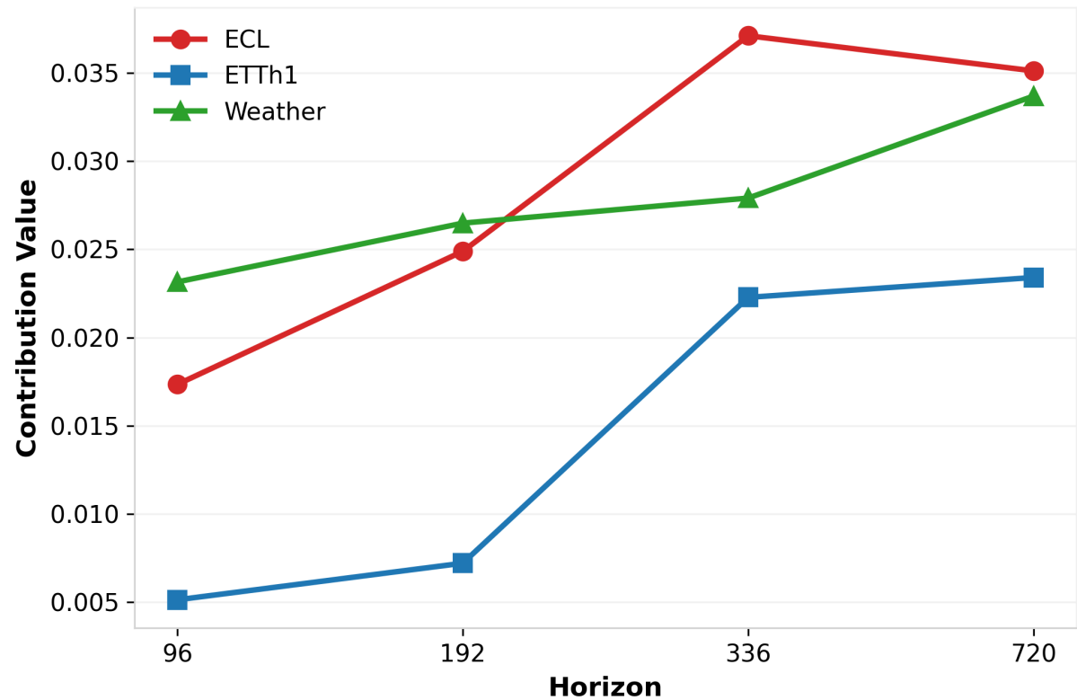
Linear Contribution
