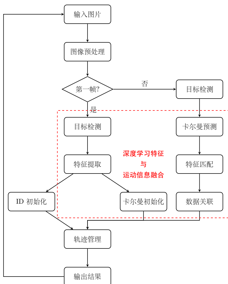
图 2-7 DeepSORT 跟踪框架
