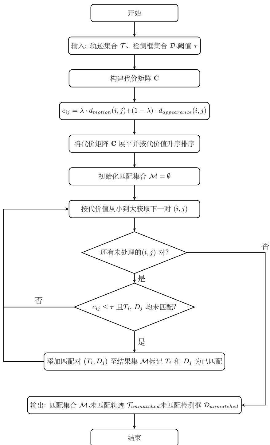
图 4-10 贪心匹配
