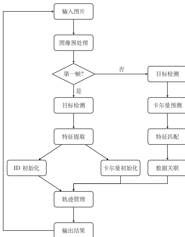
图 2-7 DeepSORT 跟踪框架
