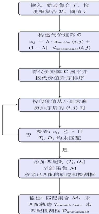
图 4-10 贪心匹配
