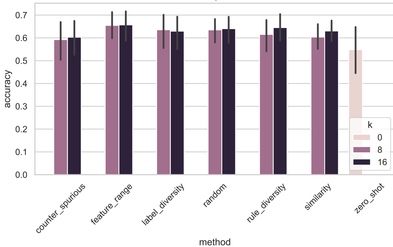
k-sensitivity: real arm
