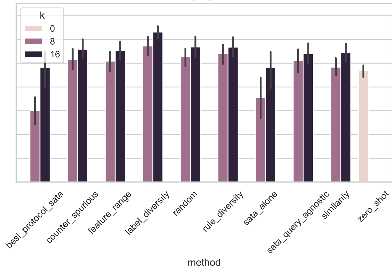
k-sensitivity: synthetic arm
