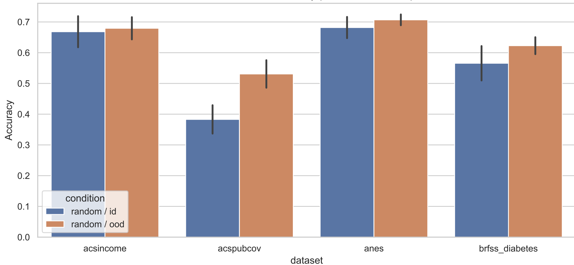
RQ1: ID vs OOD accuracy (zero-shot, random-k)
