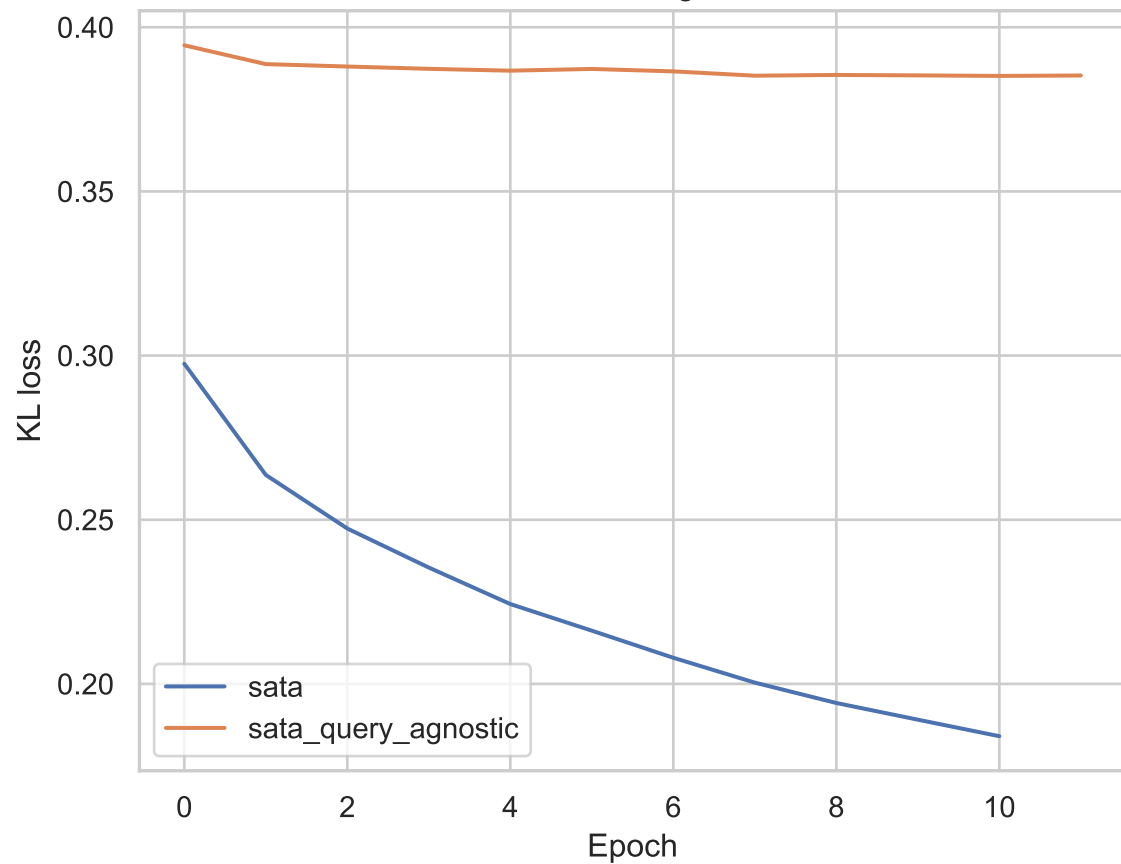
SATA training loss
