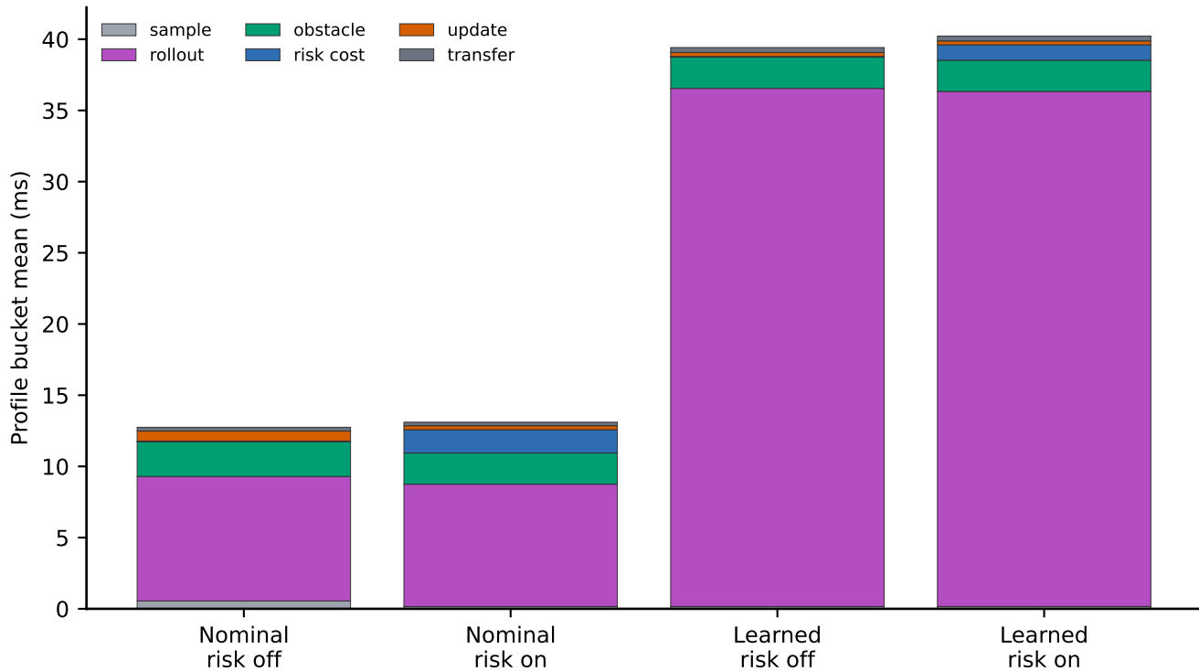
Runtime bucket breakdown: 10ep x 10step closeout
