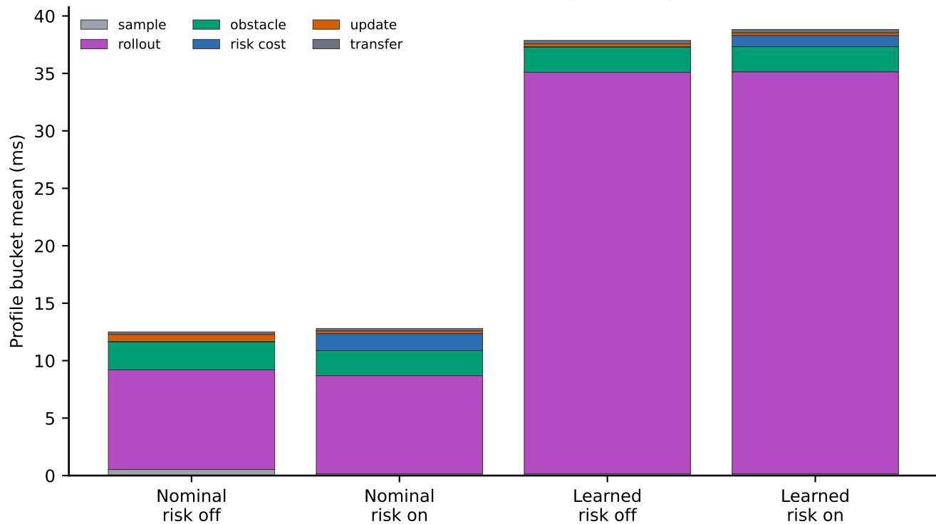
Runtime bucket breakdown: 10ep x 10step closeout
