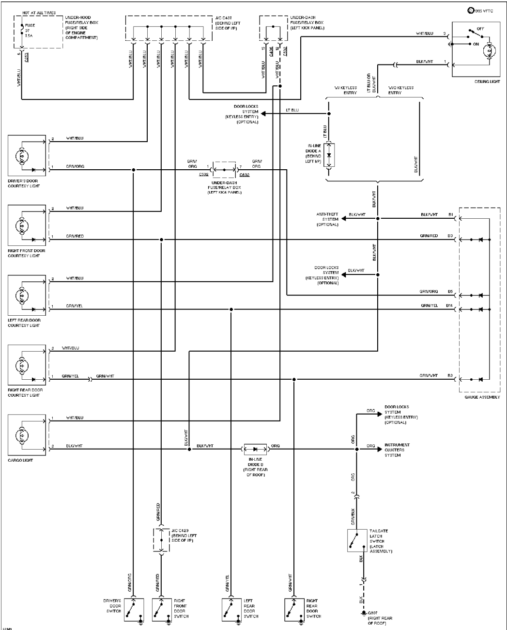
Courtesy Lamp Circuit, Wagon
