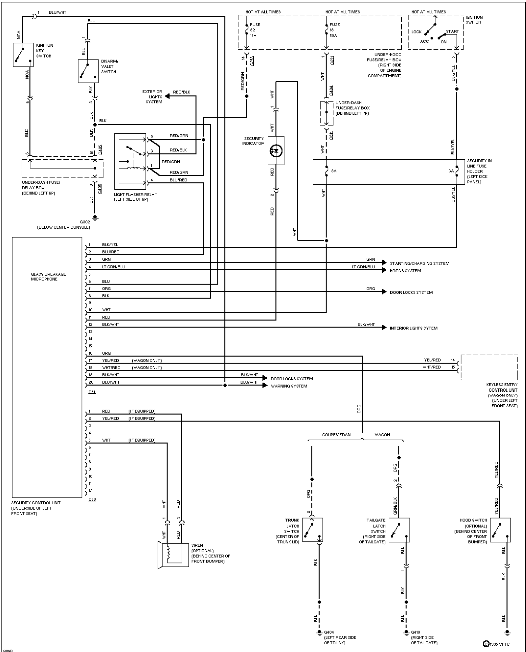
Anti-theft Circuit
