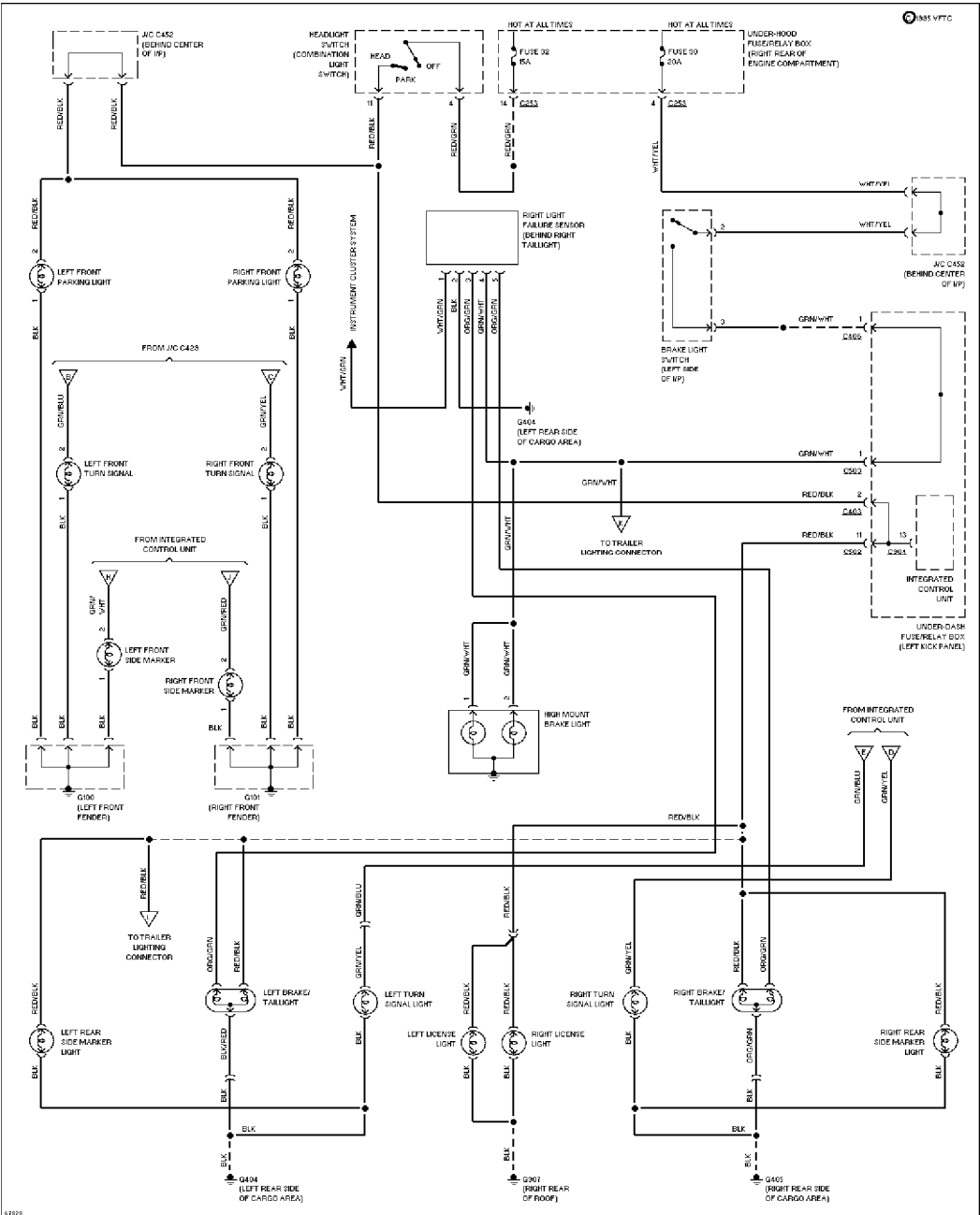
Exterior Light Circuit, Wagon (1 of 2)
