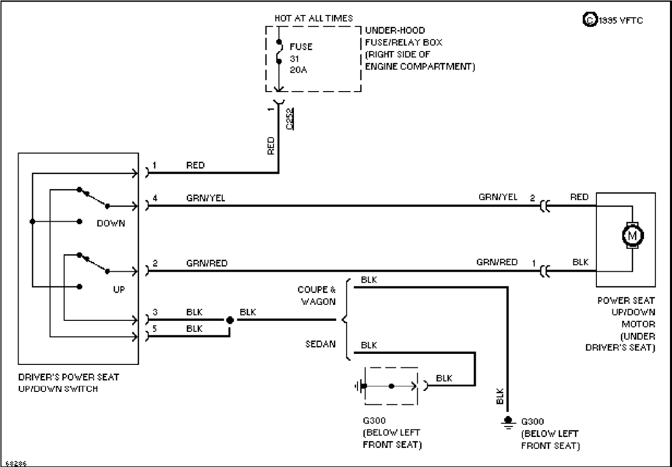
Driver Power Seat Circuit
