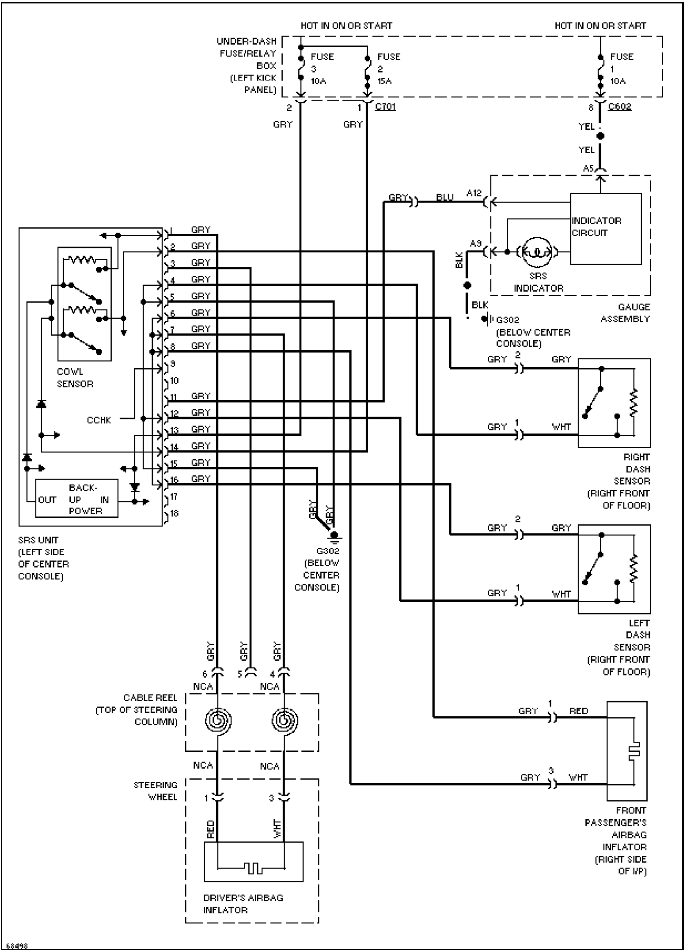
Supplemental Restraint Circuit
