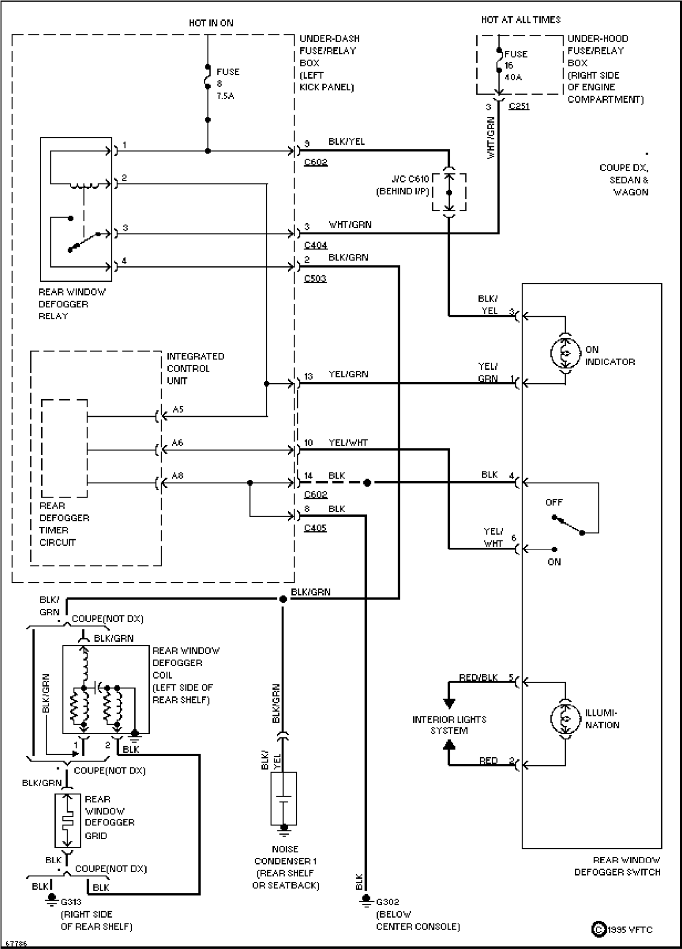
Defogger Circuit
