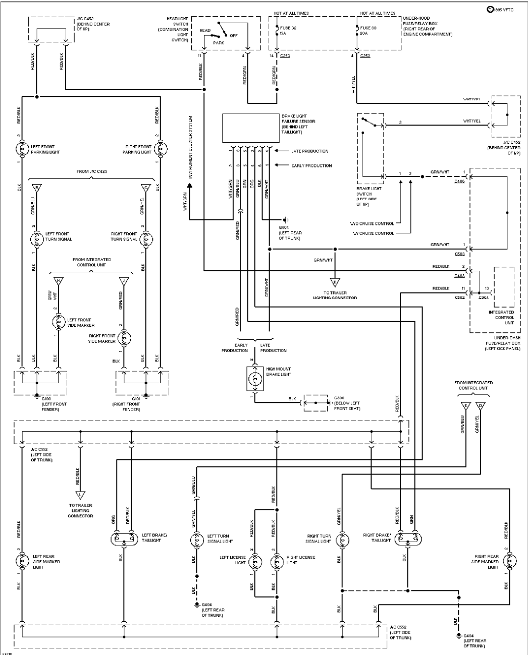
Exterior Light Circuit, Coupe & Sedan (1 of 2)
