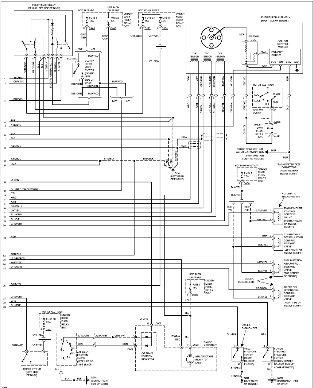
2.2L, Engine Performance Circuits (2 of 2)
