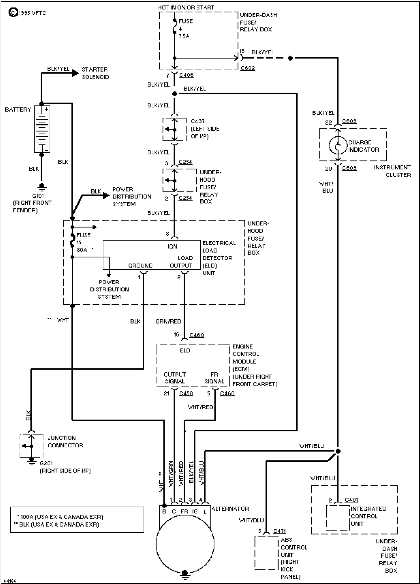
Charging Circuit
