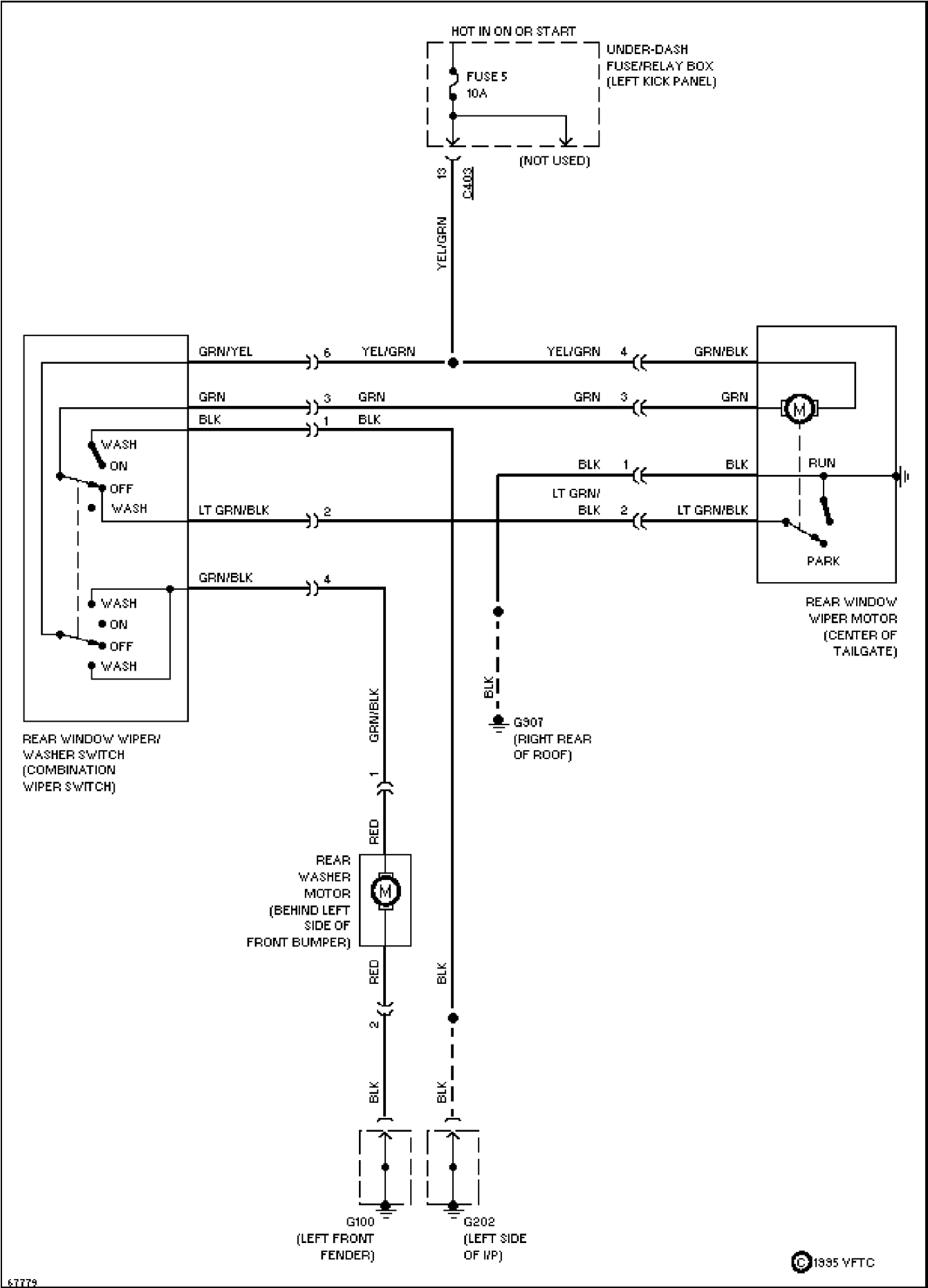
Rear Wiper/Washer Circuit
