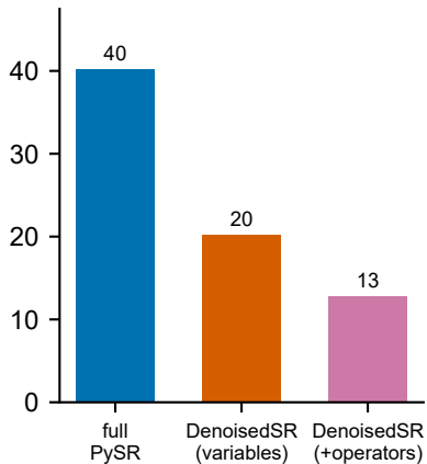
Search vocabulary
