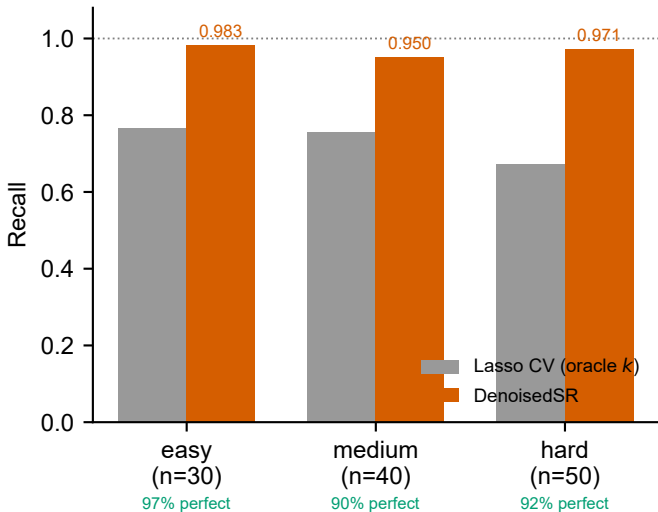
External SRSD-Feynman benchmark (never trained on)
