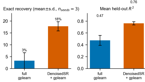
Fig. 10. Same gain transfers to a second backend. Exact recovery and mean held-out R^2 on the 30-equation Feynman subset with the gplearn backend 25 (20 generations, population 500, \sim 20 distractors; mean \pm s.d. over three random seeds). Full gplearn rarely recovers a law exactly ( 3.3 \pm 3.3\% ); supplied with the DenoisedSR variable prior over the same 3.4 predicted columns it recovers 17.8 \pm 1.9\% exact, raising mean held-out R^2 from 0.48 to 0.76.
