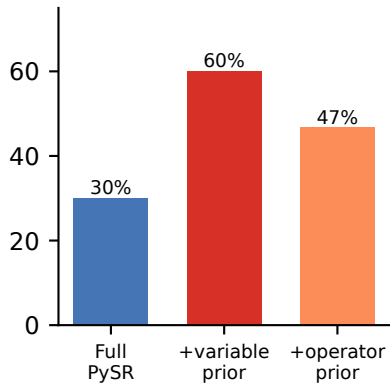
Exact recovery (n=30)
