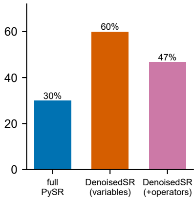
Exact law recovery (n=30)
