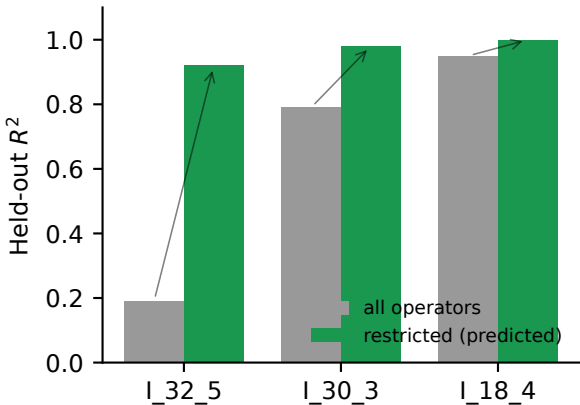
Operator restriction rescues pathological fits
