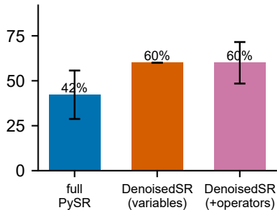
Exact recovery (n=30, 3 seeds)
