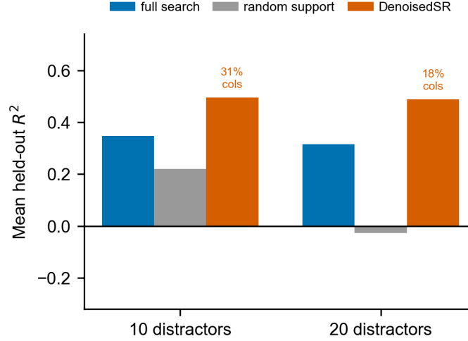
Fig. 8. The gain is search guidance, not fewer columns. Mean held-out R^2 on 24 PMLB/SRBench black-box tasks (three seeds, fixed 5 s budget) at 10 and 20 distractor variables. At matched, reduced column count (labels show columns relative to full search) DenoisedSR improves over full search while a same-size random support degrades far below it.
