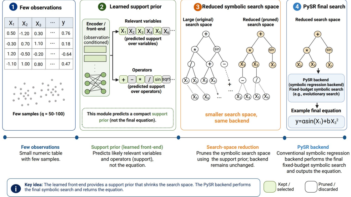
Fig. 1. DenoisedSR narrows the symbolic-regression search space. From a small set of observations the learned front-end predicts a compact support prior (relevant variables and, optionally, operators); a conventional symbolic-regression backend then performs the final search over the reduced space and returns a verifiable equation. The neural model proposes where to look; the backend decides what the law is.
