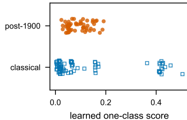
e All 128 view scores
