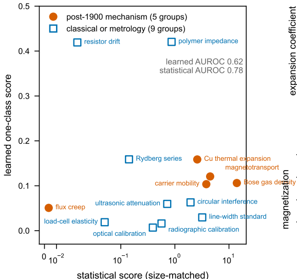
a Real NIST measurements, frozen components
