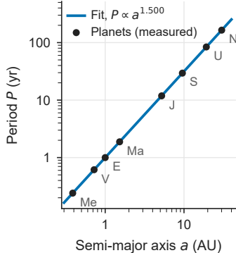
a Solar-System orbits
