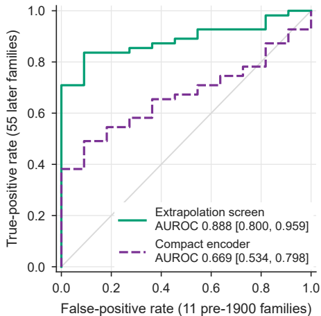
b Extrapolation screen and compact encoder
