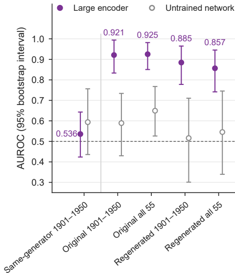
a Trained and untrained network by control set
