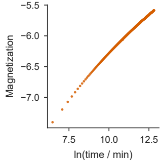
d Magnetization relaxation
