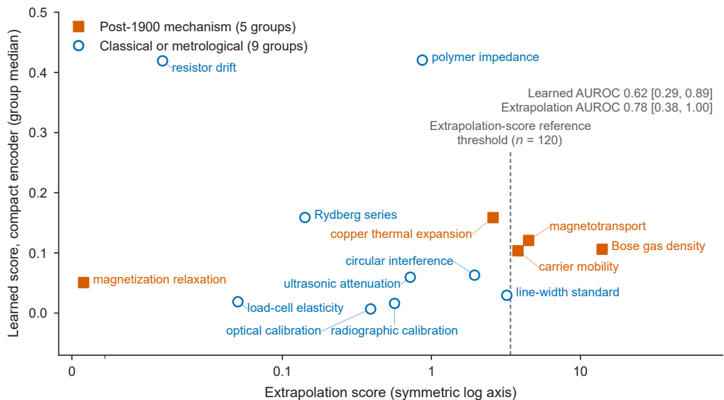
a Sixteen NIST series in 14 mechanism groups
