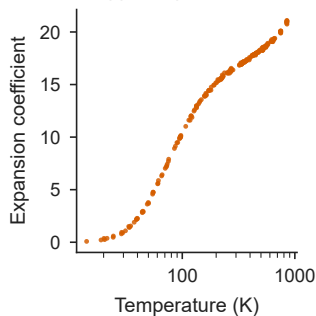
b Copper expansion
