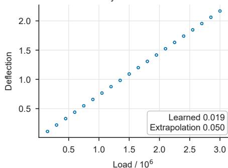
Load-cell elasticity
