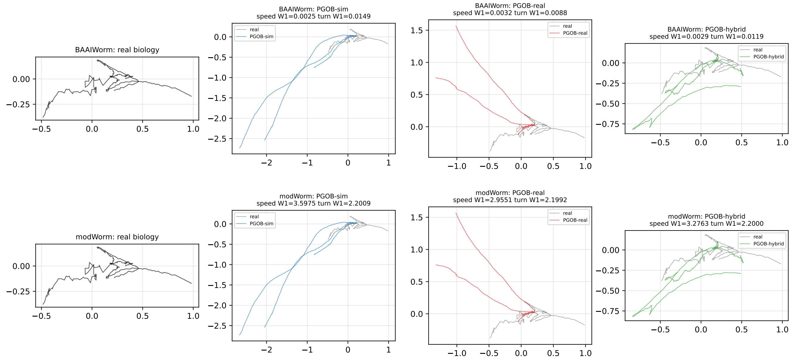
Fig 3 | Worm: real vs 3 PGOB deployment modes (BAAIWorm + modWorm, 8 panels)
