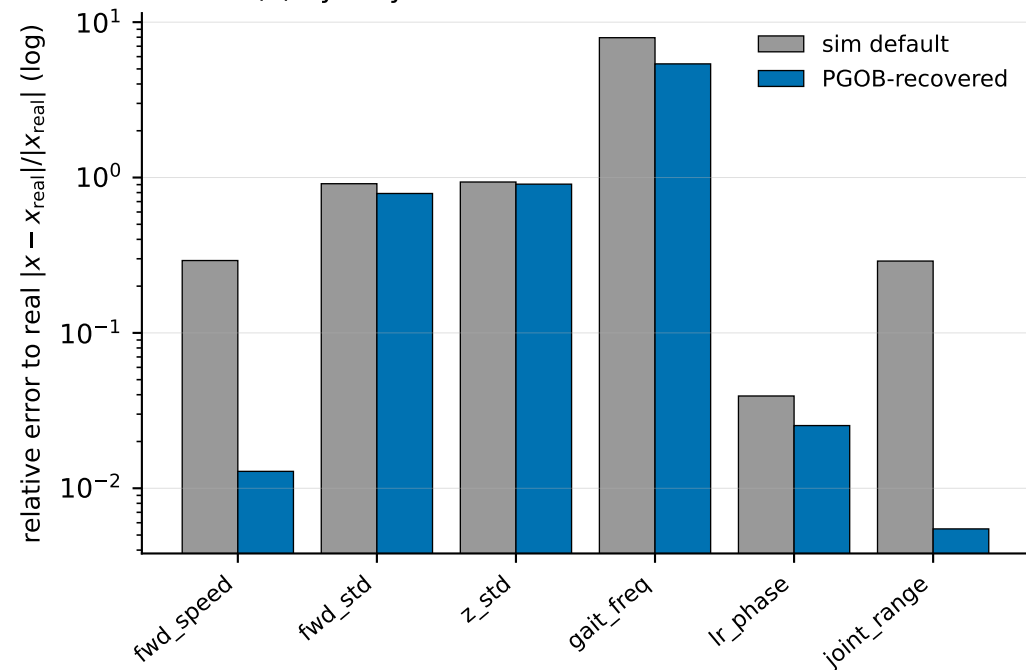
(a) flybody — recovered closer on 6/6 channels
