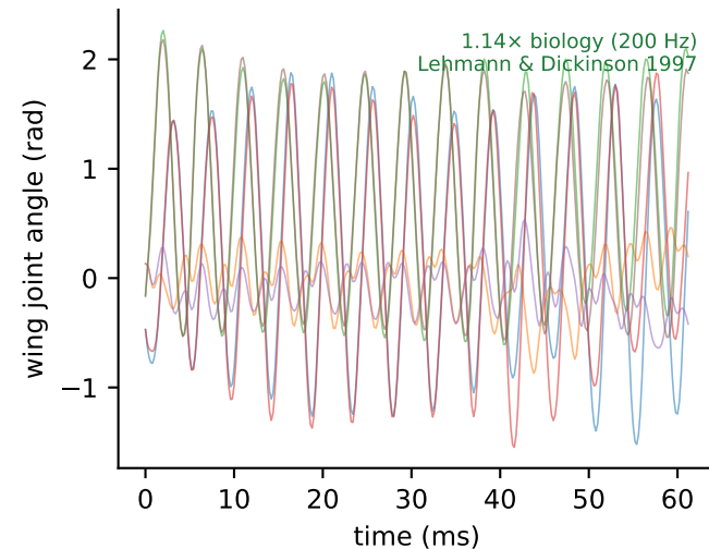
c PGOB recovered rollout (227.9 ± 5.6 Hz wing-beat)
