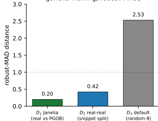
f Three-distance hierarchy (Janelia walking, robust-MAD)
