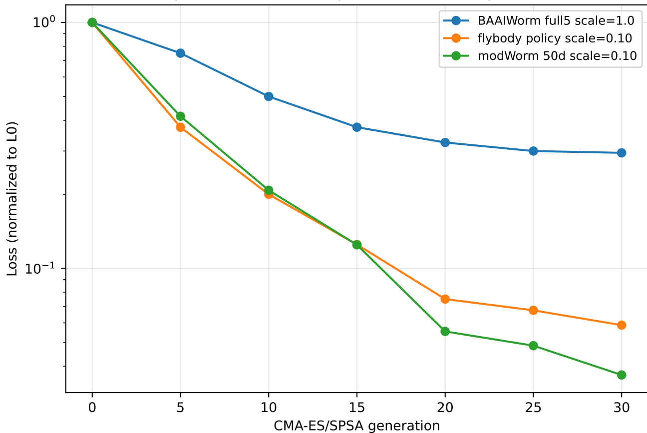
Fig 4: Cross-simulator parameter recovery curves
