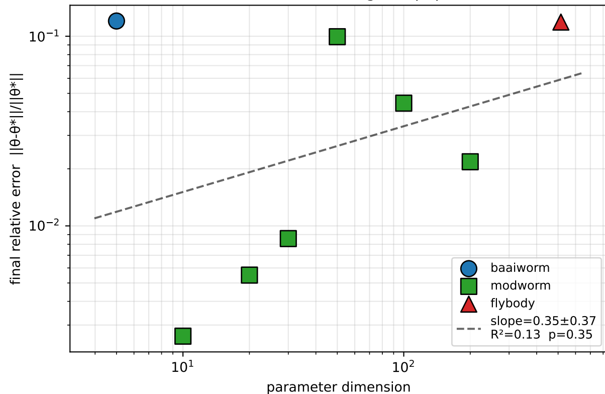
Universal scaling (n=8): dim vs final relative error (CMA-ES, scale=0.10, 30 gens, popsize=16)
