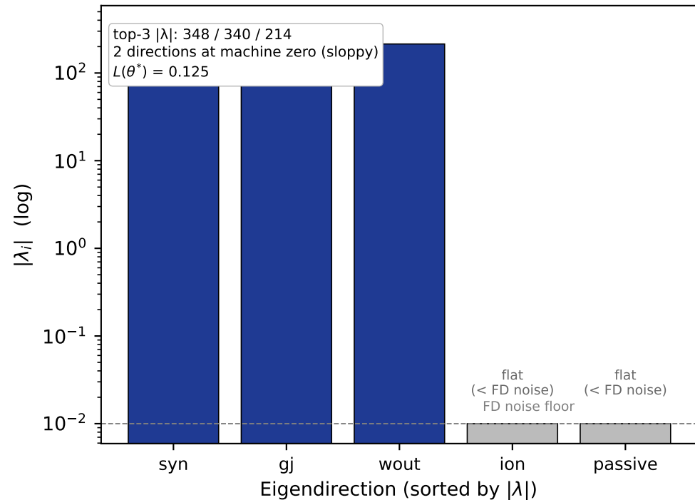
a BAAIWorm full5 Hessian spectrum at \theta^*
