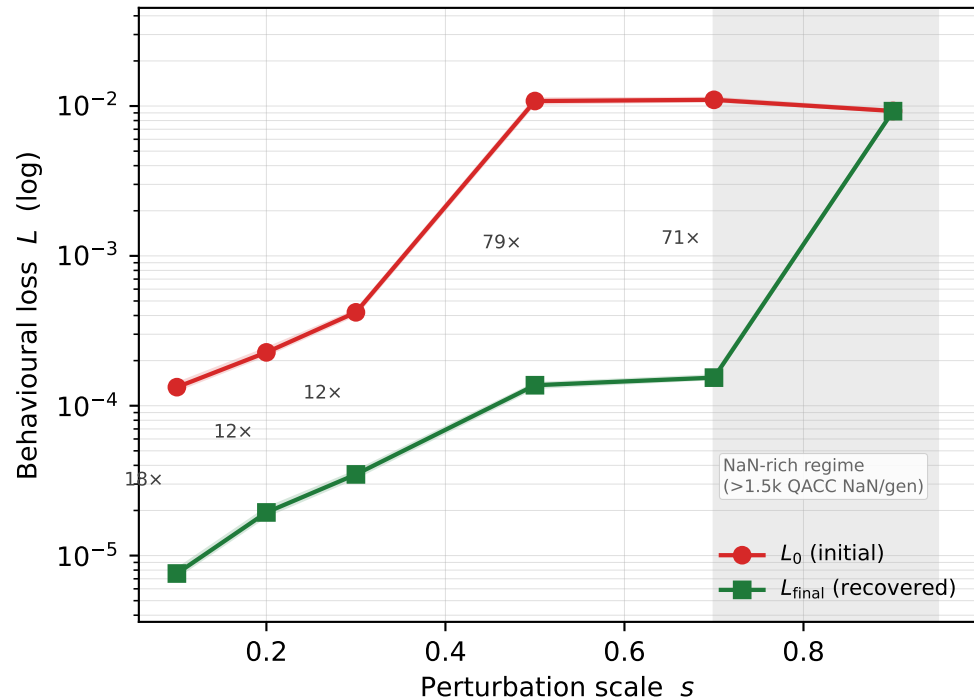
b flybody CMA-ES recovery across perturbation scales
