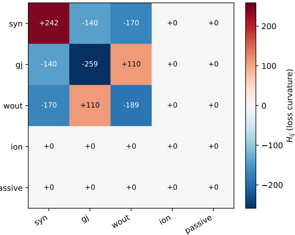
A. 5x5 Hessian at SOTA \theta^*=1 signed eigenvalues ( |\cdot| desc): +348, -340, -214, +0, +0
