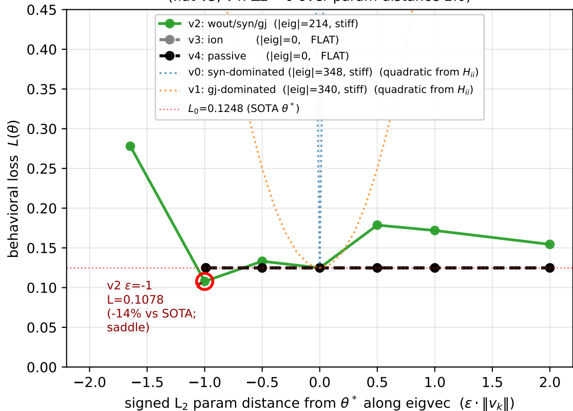
B. Direct manifold measurement: L along each Hessian eigvec (flat v3, v4: \Delta L = 0 over param distance 2.0)
