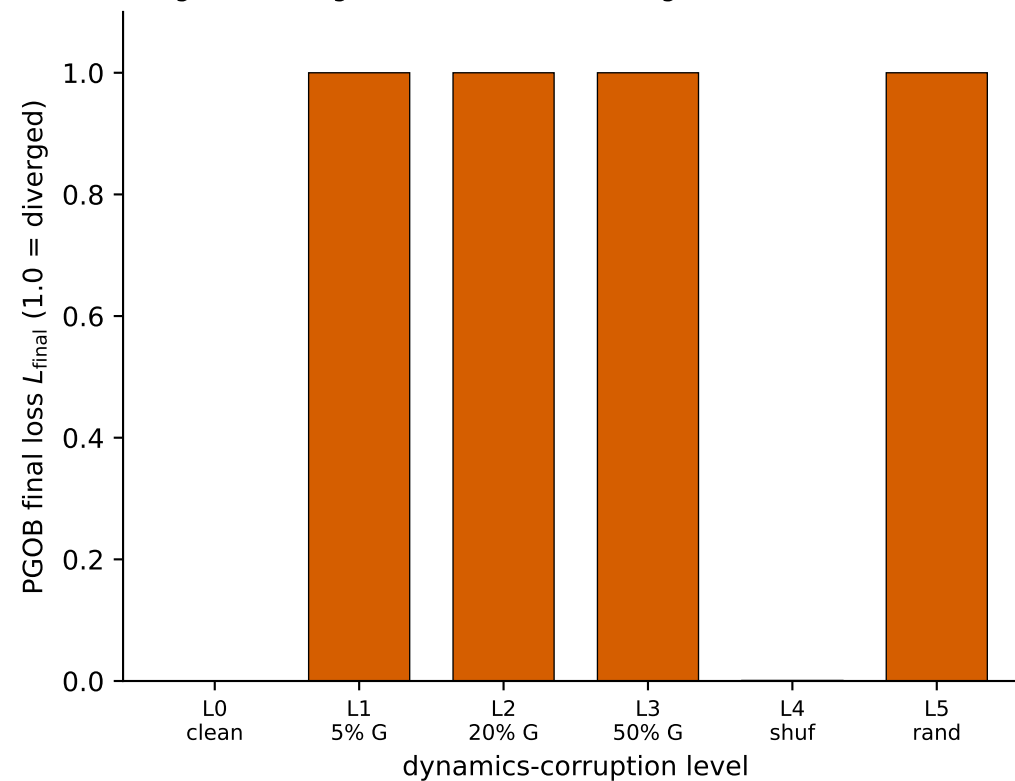
B FlyGym (MuJoCo, 126-D) -- DYNAMICS space integrator diverges on 4/6 levels; nothing to recover
