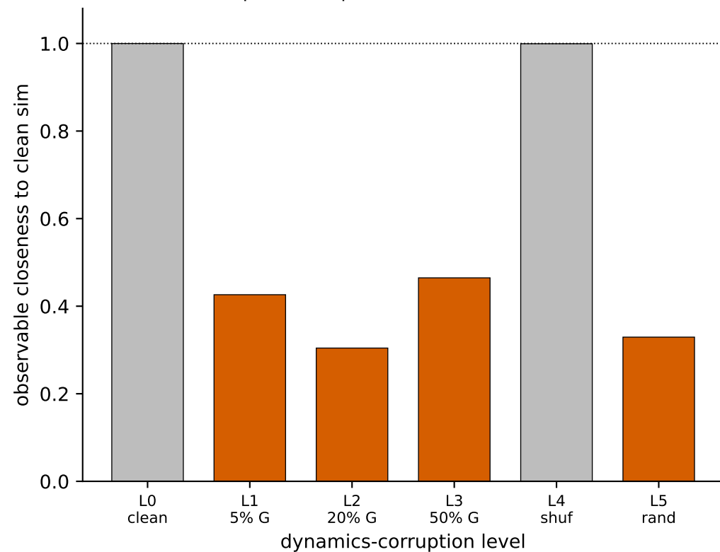
A modWorm (Cook ODE, 7-D) -- DYNAMICS space state-noise corruption collapses behaviour to 0.30-0.46
