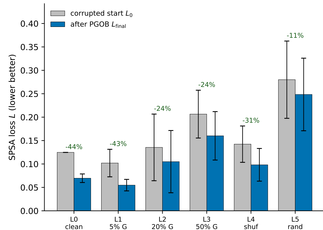
C BAAIWorm (NEURON 200-cell) -- PARAMETER space 30/30 cells L_{\text{final}} < L_0 , mean \Delta L/L_0 = -29.4\% (6 levels x 5 seeds)
