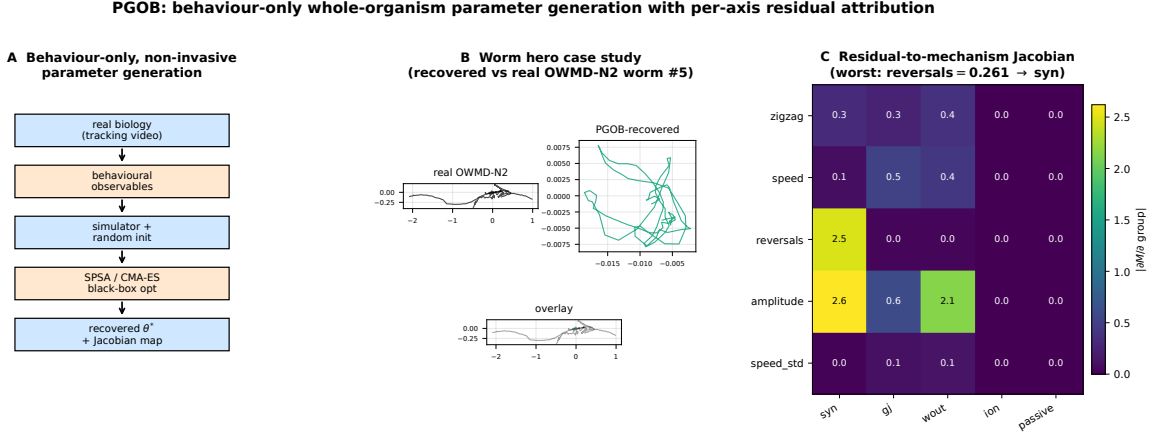
Figure 9: PGOB: behaviour-only parameter generation with per-axis residual attribution.
