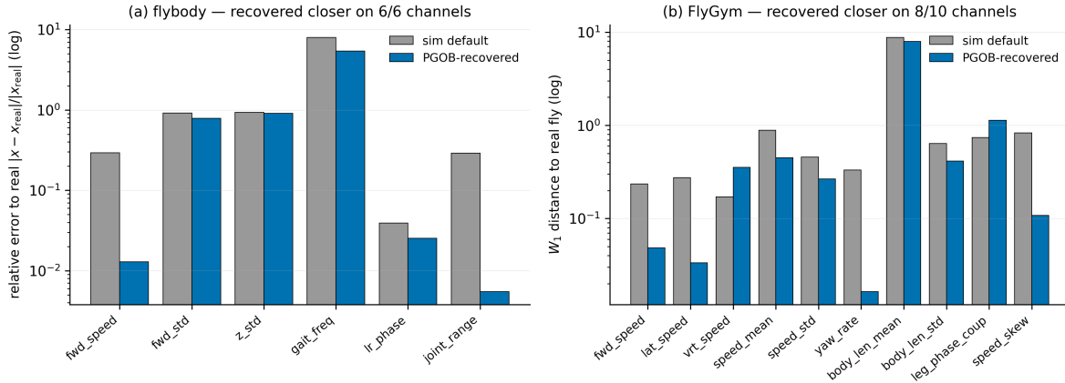
Figure 4: Real-calibration feature comparison: PGOB-recovered vs. simulator default. Per-channel distance to the real organism (log scale, lower = closer) for the simulator default (grey) and the PGOB-recovered parameters (blue). (a) flybody: relative error |x - x_{\text{real}}|/|x_{\text{real}}| of each native walking feature against the MoCap reference; the recovered bar is below the default on all six channels. (b) FlyGym: per-observable Wasserstein-1 distance to the real Janelia fly; the recovered bar is below the default on eight of ten channels. BAAIWorm and modWorm are not plotted here: the worm real-calibration evidence is the rigorously powered hero panel (PGOB-real D_1=0.71 vs. sim default D_3=21.82 to OWMD-N2, main text) and the modWorm native channels divide by near-zero real values that make a per-channel relative-error panel uninterpretable.
