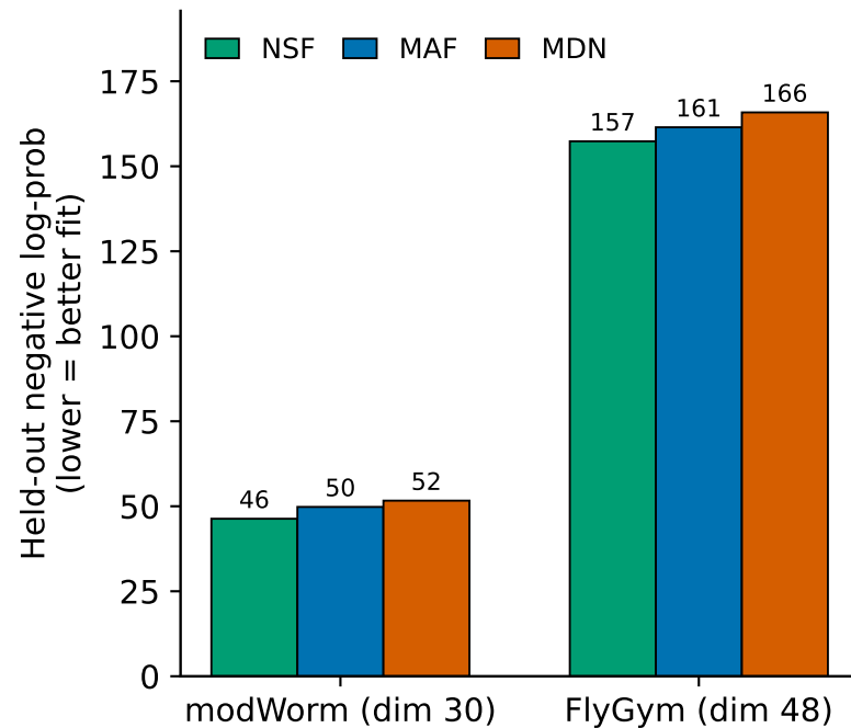
B Density-estimator comparison: NSF > MAF > MDN
