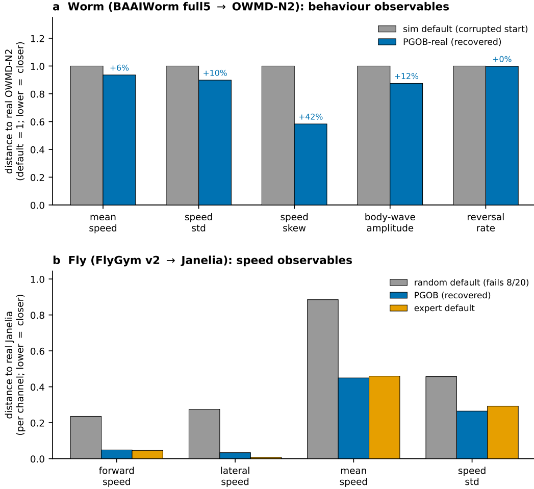
Figure 1: Behaviour-observable read of PGOB generation (worm and fly). Each bar is one behavioural observable; lower = closer to the real reference. a , Worm (BAAIWorm full5 → OWMD-N2): per-observable distance to real OWMD-N2, normalised so the deposited (corrupted-weight) default = 1 in each channel, against the PGOB-generated worm (blue); annotations give the PGOB reduction. PGOB is closer to real on all five headline observables shown (mean speed, speed std, speed skew, body-wave amplitude, reversal rate) and on 7/10 of the full observable set (aggregate W_1 3.91 → 3.42). b , Fly (FlyGym v2 → Janelia, N=20 /arm): per-channel distance to real Janelia for the random actuator-gain default (grey; fails to walk 8/20), the PGOB-generated controller (blue), and the expert default (orange). The PGOB bars collapse onto the expert bars on the speed channels, closing 98.7% (forward) and 90.4% (lateral) of the random-to-expert gap.
