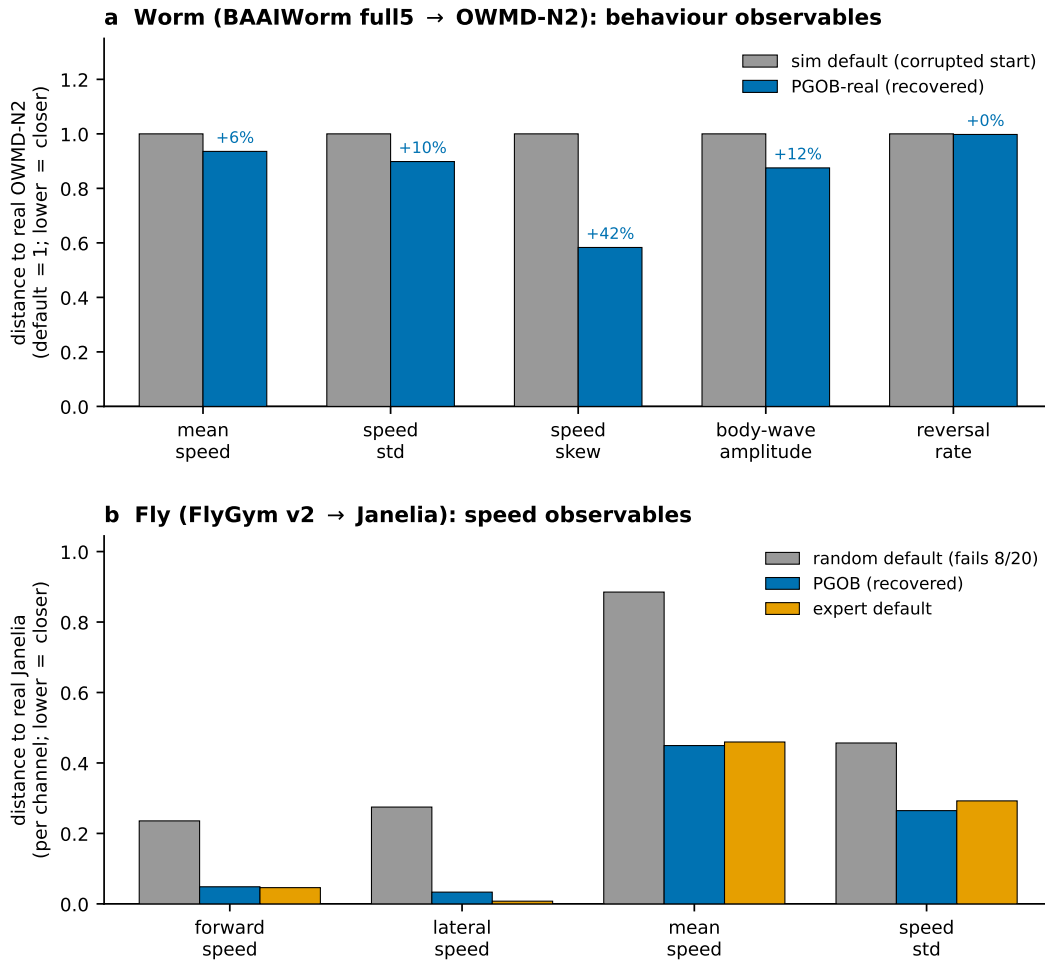
Figure 1: Behaviour-observable read of PGOB generation (worm and fly). Each bar is one behavioural observable; lower = closer to the real reference. a , Worm (BAAIWorm full5 \rightarrow OWMD-N2): per-observable distance to real OWMD-N2, normalised so the deposited (corrupted-weight) default = 1 in each channel, against the PGOB-generated worm (blue); annotations give the PGOB reduction. PGOB is closer to real on all five headline observables shown (mean speed, speed std, speed skew, body-wave amplitude, reversal rate) and on 7/10 of the full observable set (aggregate W_1 3.91 \rightarrow 3.42 ). b , Fly (FlyGym v2 \rightarrow Janelia, N=20 /arm): per-channel distance to real Janelia for the random actuator-gain default (grey; fails to walk 8/20), the PGOB-generated controller (blue), and the expert default (orange). The PGOB bars collapse onto the expert bars on the speed channels, closing 98.7% (forward) and 90.4% (lateral) of the random-to-expert gap.
