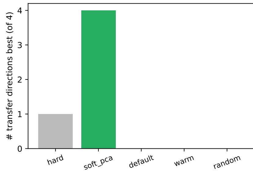
C. five-init grid: soft_pca best 4/4 (18/20 cells filled)
