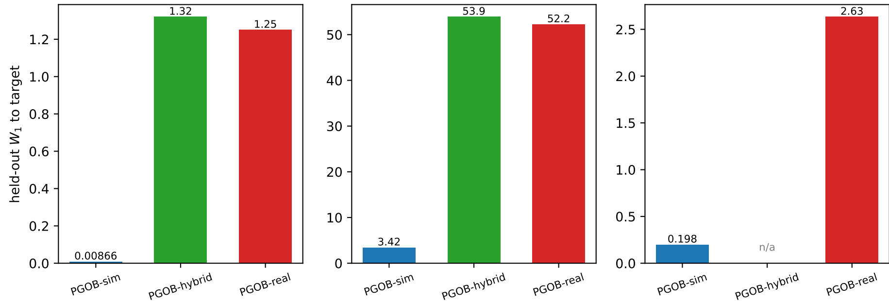
Three genuine PGOB modes: sim behaviour recoverable, real hits an irreducible sim \leftrightarrow real gap
