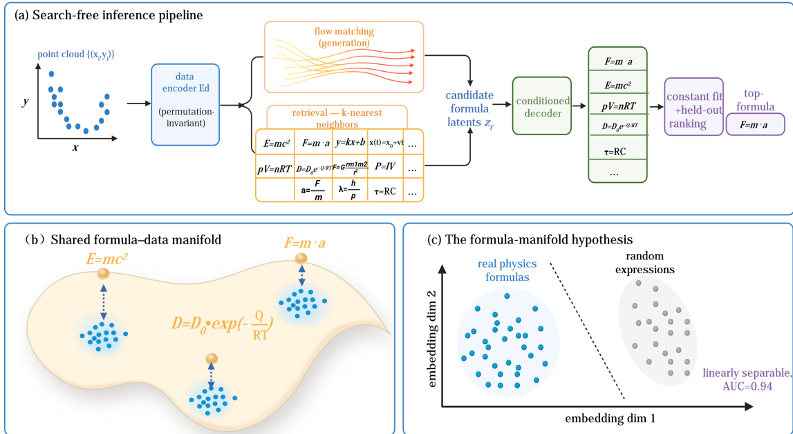
Figure 1 | PISR overview. (a) Search-free inference pipeline: a point cloud is embedded by a permutation-invariant data encoder; a flow-matching field generates candidate formula latents z_f and
